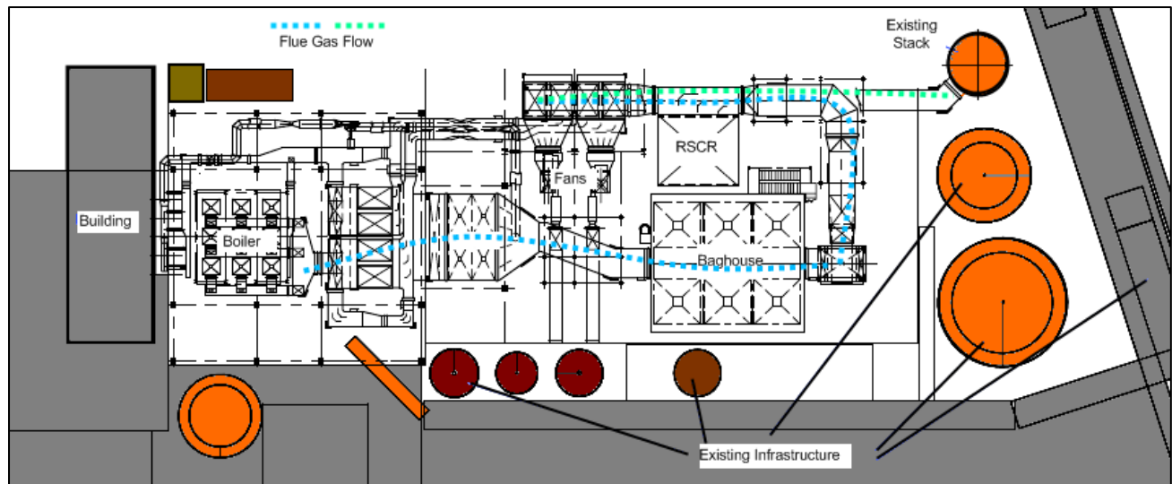
Figure 9: Boiler and AQS Arrangement Within Existing Infrastructure
