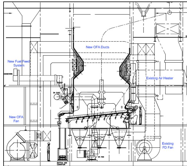
Figure 8: Air Duct Arrangement for Biomass Conversion
