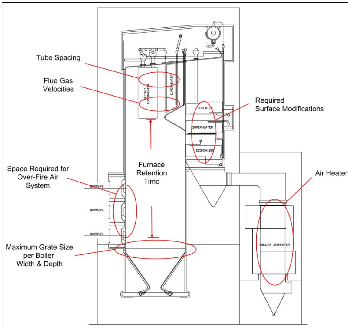
Figure 3: Evaluating A Biomass Conversion, Marking Important Areas of Evaluation for Converting A Unit to Fire Biomass
