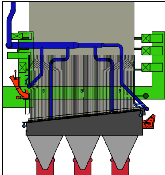
Figure 4: Typical Modifications to the Furnace Include an Over-Fire Air System, Addition of a Grate and Ash Hoppers, Fuel Distributors
