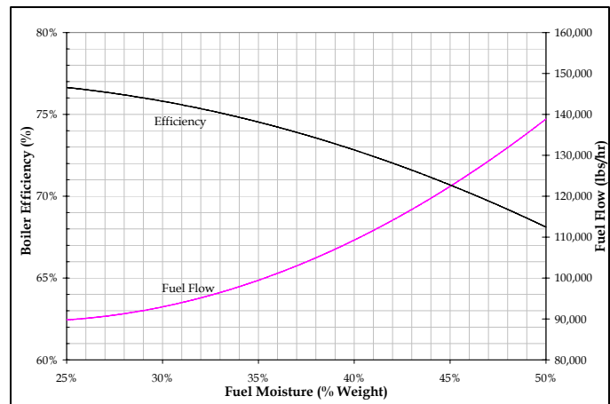
Figure 2: Fuel Moisture vs. Efficiency
